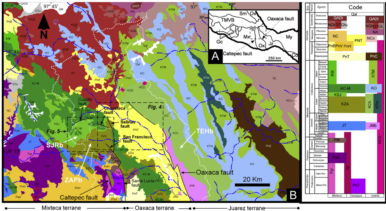
Figure 3. Simplified map of the regional geology of south-central México from Martínez-Amador et al. (2001). A: Structural terranes that form continental southern México according to Keppie (2004). The SMS is formed by the Guerrero Composite terrane (Gc), Mixteca (Mx), Oaxaca (Ox) and Juarez (Jz) terranes. The nearby Trans Mexican Volcanic Belt (TMVB), Sierra Madre (Sm), Maya (My) and Chortis (Co) terranes are also outlined. B: Summarised geology of the north sector of the SMS re-drawn from Martínez-Amador et al. (2001), and location of the SJRb, ZAPb and TEHb-white dotted line. PrO: multi-deformed basal Oaxaca complex; PaA: Acatlán basal metamorphic complex; PM: continental sedimentary Matzitz Fm; Pgr: granite Caltepec and Totoltepec formations; Jgr: anatectic lower Jurassic granite; JT: sandstone and andesitic tuff, Tecomazuchil Fm; JMb: mylonitic belt; KZA: lutite-limestone, Zapotitlán Fm; KCh: sandstone, Chivillas Fm; KTM: lutite-limestone Tamaulipas Fm; KSJ: lutite-sandstone, San Juan Raya Fm; KC-M: limestone Cipiapa/Miahuatepec Fm; KO: limestone-dolomite, Orizaba Fm; KM: lutite-sandstone Mezcala Fm; KTM: tite-limestone, Maltrata, Mendez and Atoyac Fm; PnT: Tamazulapan Fm; PnC: lutite-sandstone Chicontepec Fm; PnB: conglomerates-sandstone Balsas Fm; PnV: limestone-conglomerates Pie de Vaca Fm; PnH: andesitic tuf-sandstone, Huajuapán Fm; PNT: conglomerates-travertine (tufa), Tehuacán Fm; NCD: monzonite-diorite; NC: conglomerate-andesitic tuff, Cuayuca Fm; NCo: sandstone-conglomerate; NA: andesite; NQb: basalt; QT: andesitic tuff-andesite; Qtu: travertine (tufa); QL: lahar; QADt: andesitic-dacitic tuff; Qal: alluvial. Dash-dot lines indicate main drainage.
