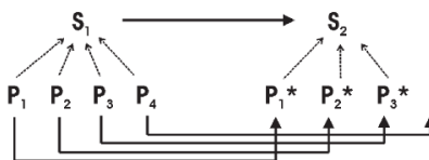
Figure 4. Fodor's (1968) diagram. To translate to our earlier terminology: each of P_1, P_2 \dots P_4 represent one microstate b_1, b_2 \dots b_N and P^*_1 is time-evolved state from P_1 (in the earlier notation: T(b) ). S_1 represents B and S_2 represents A. Earlier the arrows were uninterpreted but here we see that the vertical arrows represent supervenience relations, and the horizontal arrows represent dynamical evolution.
