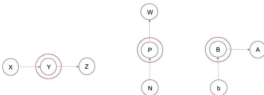
Figure 1. In each of these diagrams (causal, grounding or multi-dimensional respectively), the circled variable (or fact) screens off the less proximate ancestors (X, N and b respectively) from Z, W and A facts respectively. As such, each figure demonstrates a Markov condition.
