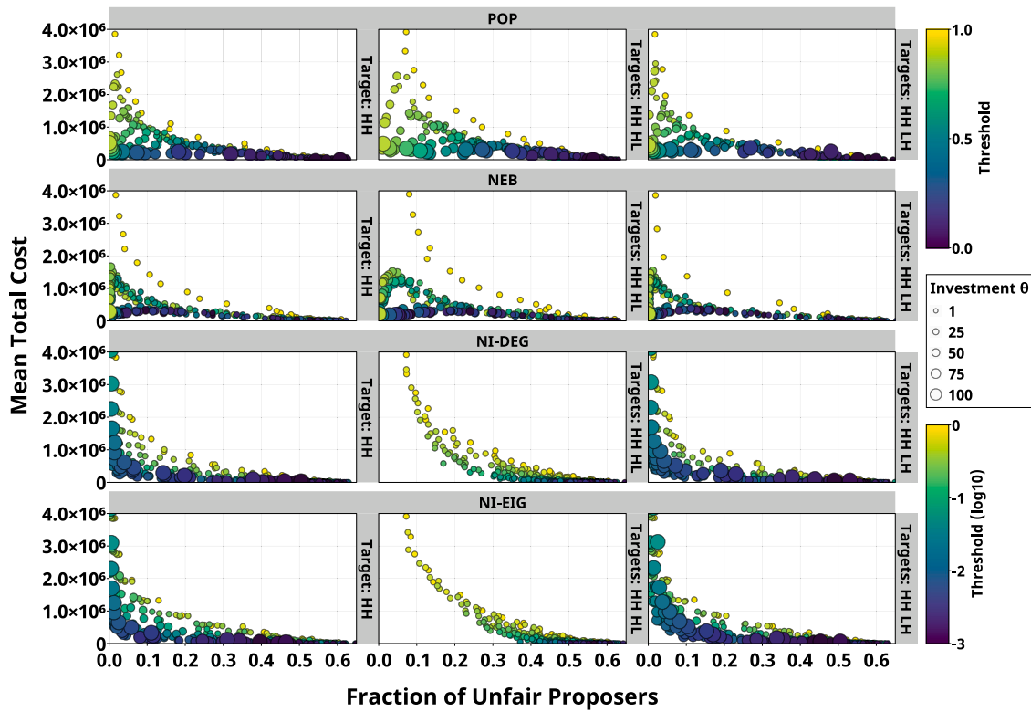
Fig. 3. Pareto fronts for each scheme in BA networks.
