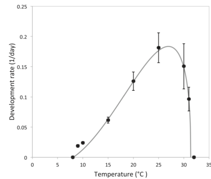
Figure 2: Temperature-dependent development rate of D. sukukii for the egg-to-pupa stage. Data were fitted with a standard model of arthropod temperature-dependent development (Brière 1999). Data points are means \pm SD.
