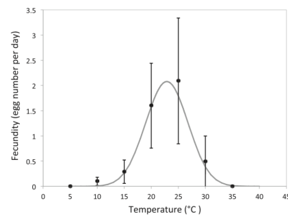
Figure 1: Temperature-dependent fecundity of D. suzukii . Fecundity is expressed as the number of eggs per female per day, as measured over a 10-d period following a 4-d acclimation period. Data were fitted using a polynomial function with compact support, adapted from Saryazdi and Cheriet (2007). Data points are means ± SD.
