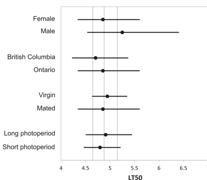
Figure 4: LT 50 s (°C) + 95% confidence limits for all group comparisons. The overlapping CIs indicate that there were no significant differences between groups. Dashed lines represent the overall LT 50 and CI 95 for the whole data set
